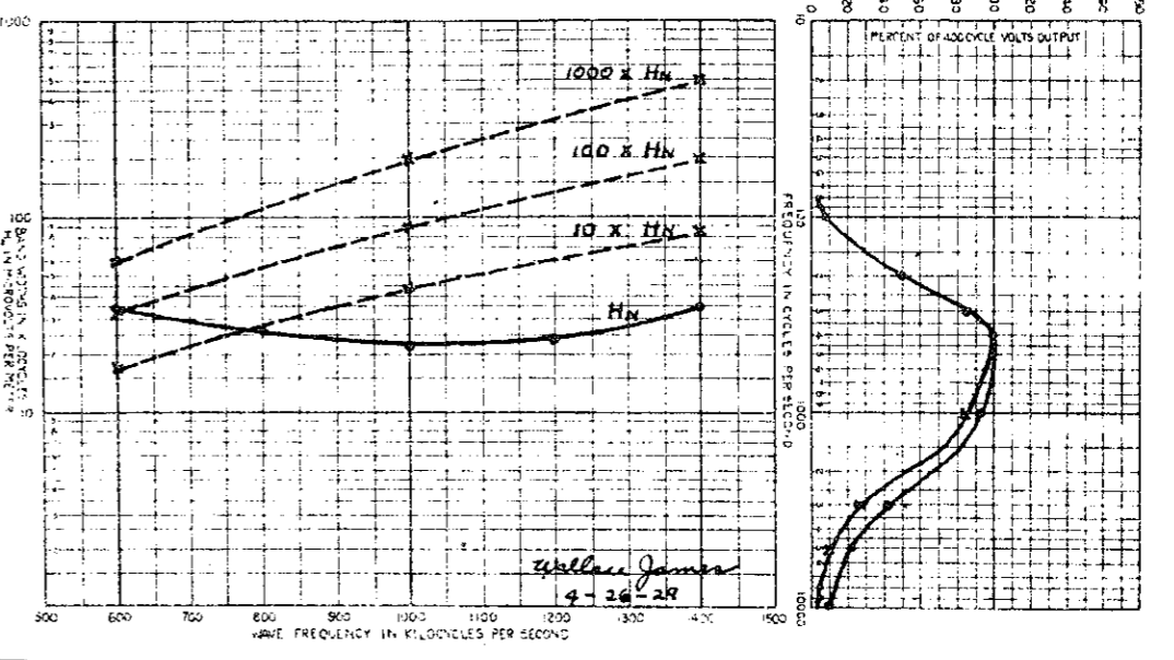
ATWATER KENT MODEL 40 MARCH 1929
